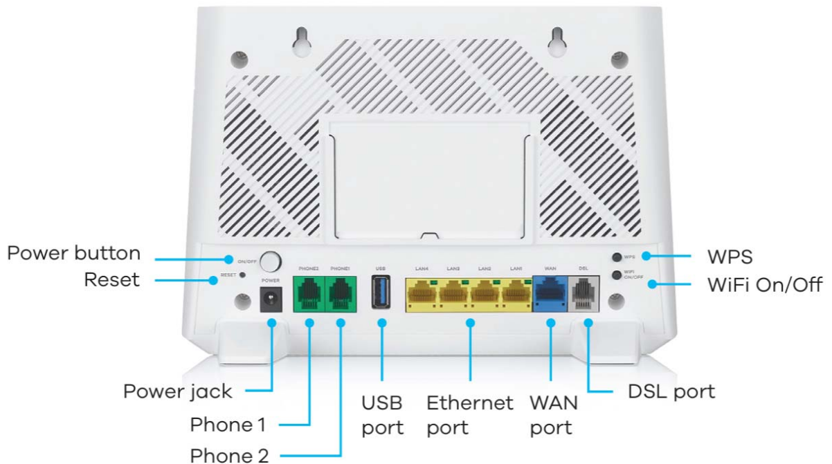
Figure 32 Rear Panel (VMG8623-T50B)
