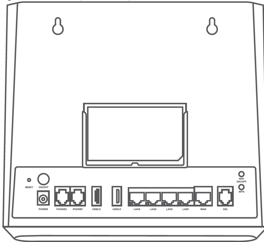
Figure 33 Rear Panel (VMG8825-T50)
