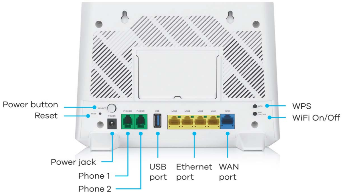
Figure 37 Rear Panel (EMG5523-T50B)
