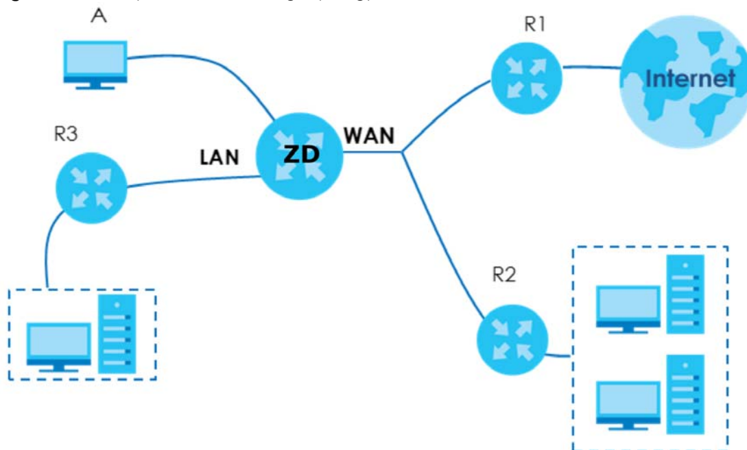
Figure 132 Example of Static Routing Topology
