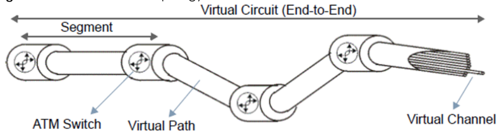
Figure 265 Virtual Circuit Topology
