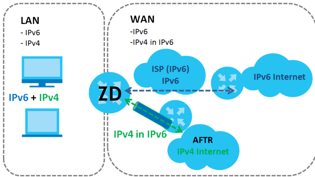
Figure 81 Dual Stack Lite
